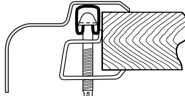
U-Channel Type Mounting System
