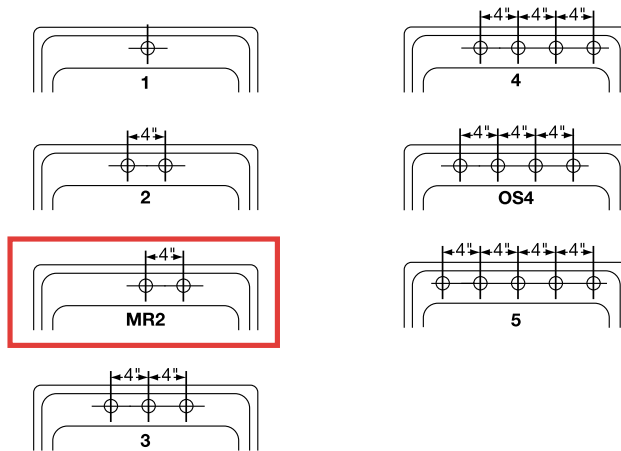
Quick-Clip® Mounting System
